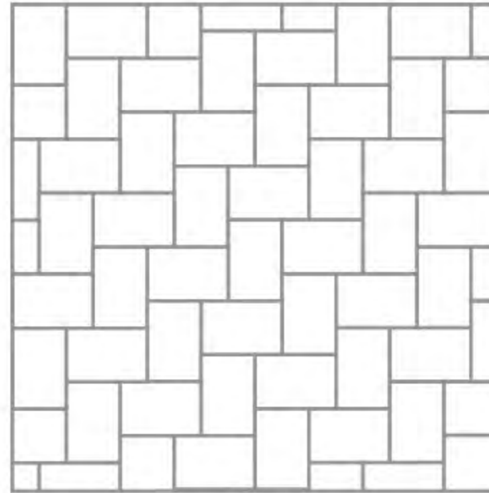
90° HERRINGBONE (6" X 9" ONLY)
