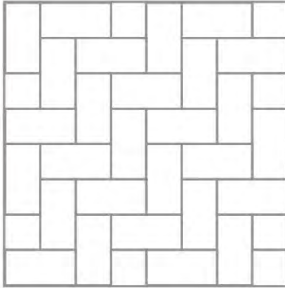
90° HERRINGBONE
